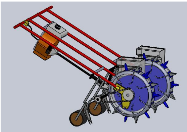
Gambar 2. Design Mesin Penanam Jagung Sistem Roda Tanjak
